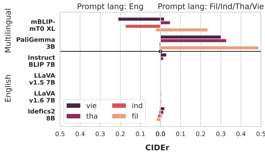
Figure 4: Existing VLMs produce subpar image captions in SEA languages.
